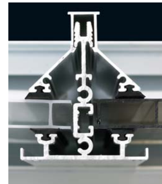
DEGLAS Patio System (DPS)
