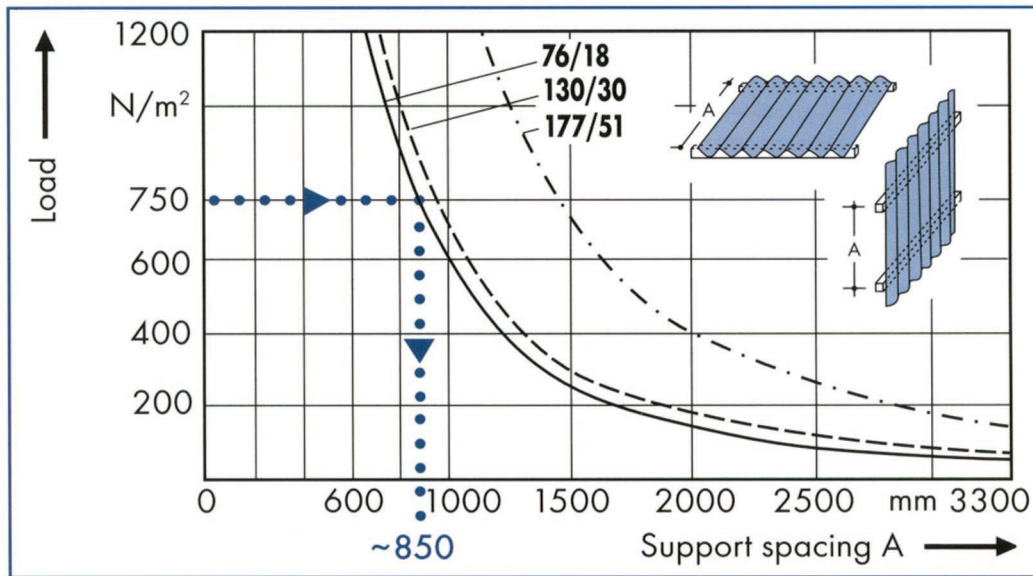
Fig. 3: Recommended Support Spacing for DEGLAS Corrugated Sheets.
